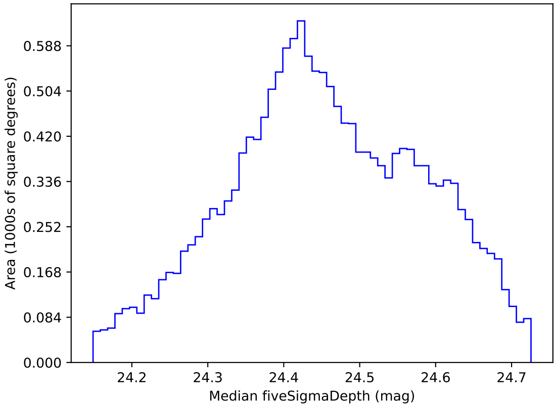
too_ignore_100_1v3.4_10yrs WFD g band: Median fiveSigmaDepth
