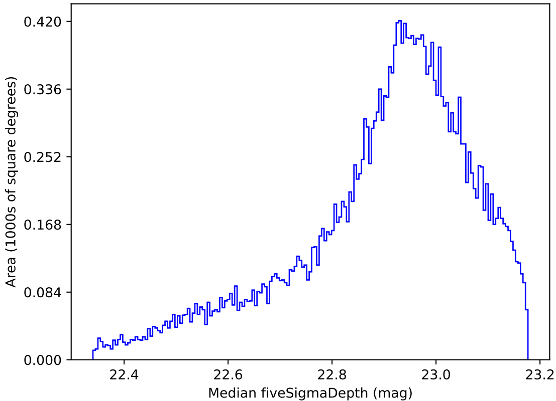
too_ignore_100_1v3.4_10yrs All sky z band: Median fiveSigmaDepth
