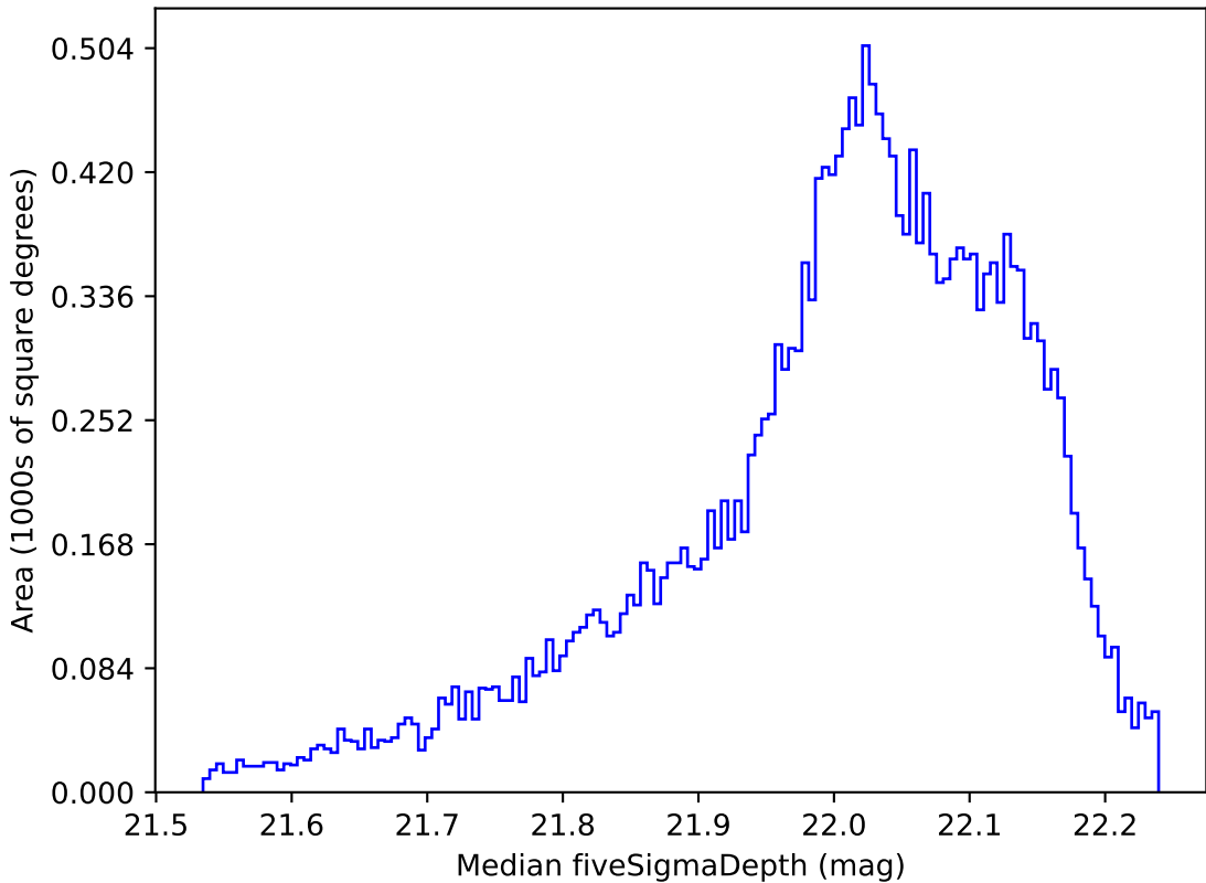
too_ignore_100_1v3.4_10yrs All sky y band: Median fiveSigmaDepth
