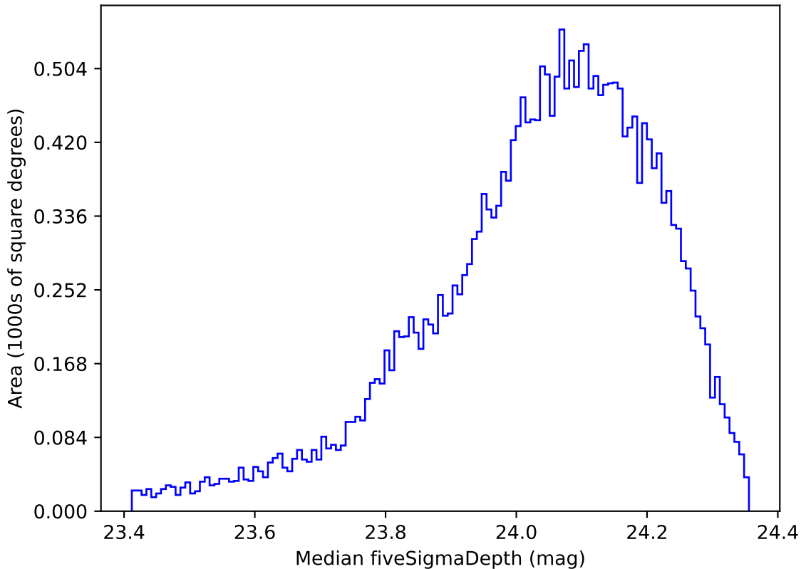
too_ignore_100_1v3.4_10yrs All sky r band: Median fiveSigmaDepth
