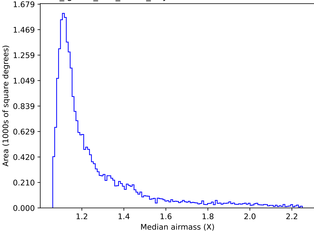
too_ignore_100_1v3.4_10yrs Yr 1 z band: Median airmass
