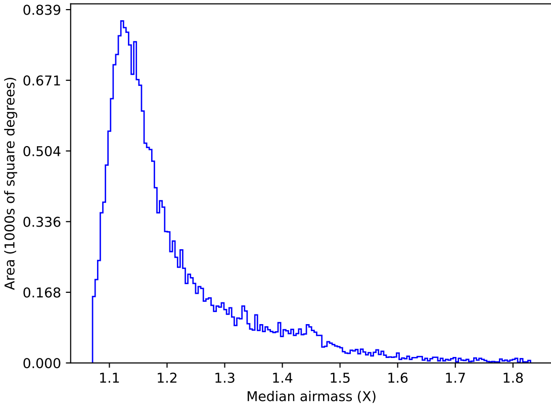
too_ignore_100_1v3.4_10yrs Yr 1 y band: Median airmass
