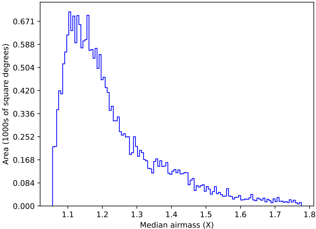
too_ignore_100_1v3.4_10yrs Yr 1 u band: Median airmass
