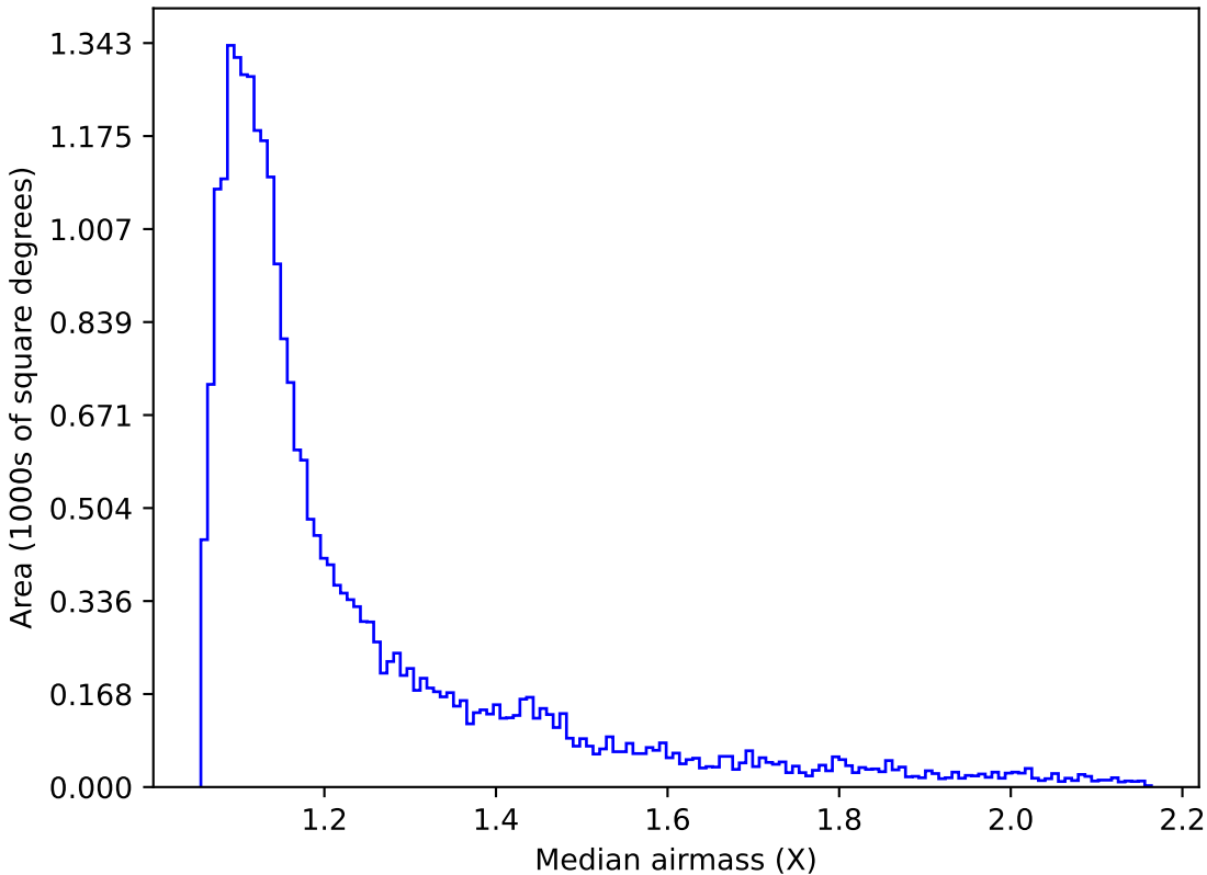
too_ignore_100_1v3.4_10yrs Yr 1 r band: Median airmass
