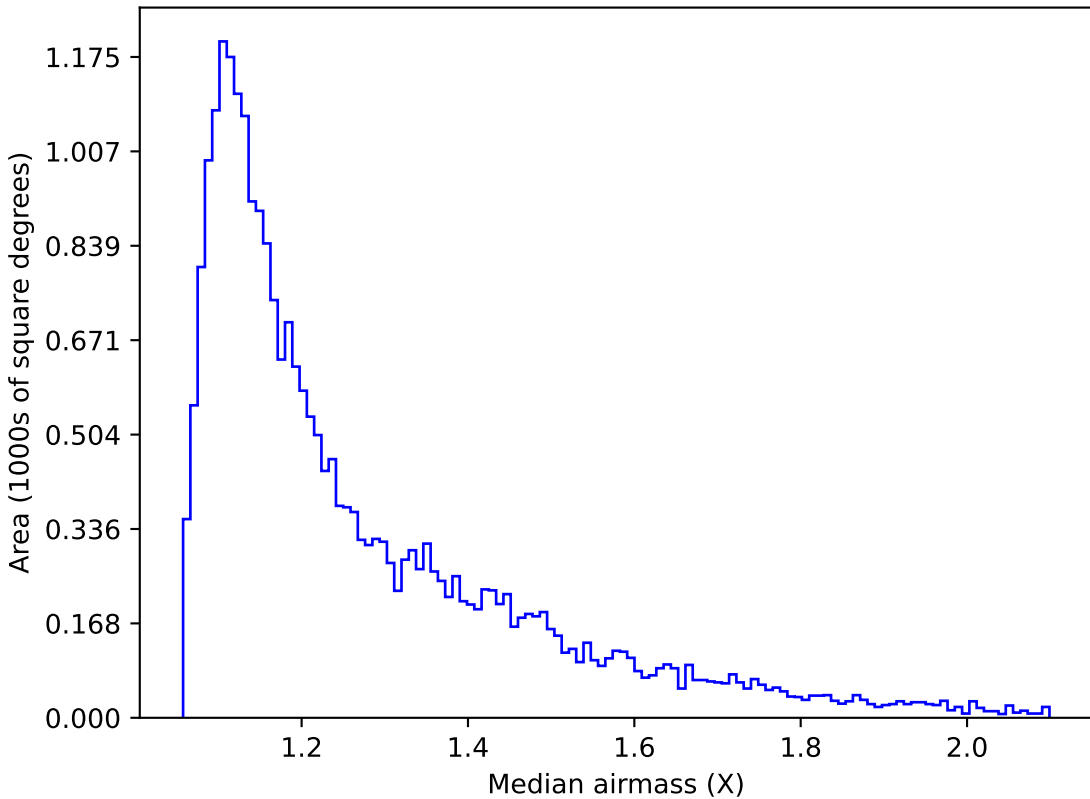
too_ignore_100_1v3.4_10yrs Yr 1 g band: Median airmass
