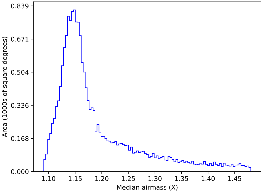
too_ignore_100_1v3.4_10yrs WFD y band: Median airmass
