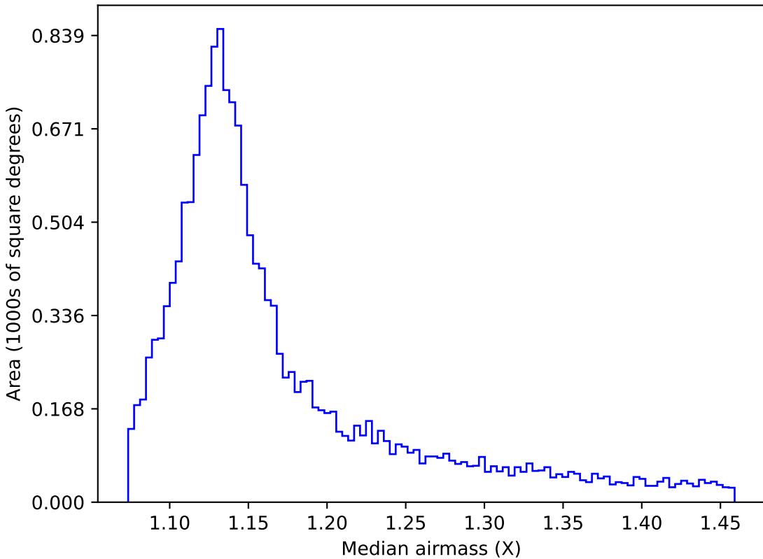
too_ignore_100_1v3.4_10yrs WFD r band: Median airmass
