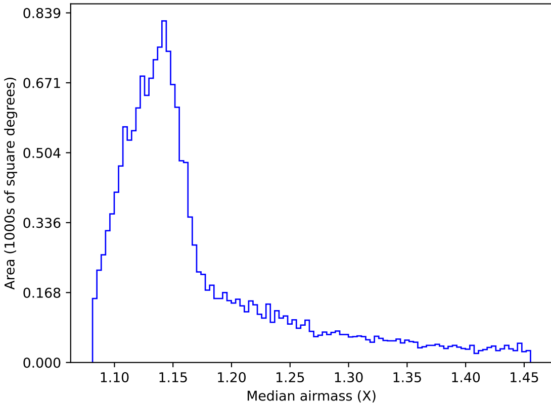
too_ignore_100_1v3.4_10yrs WFD i band: Median airmass
