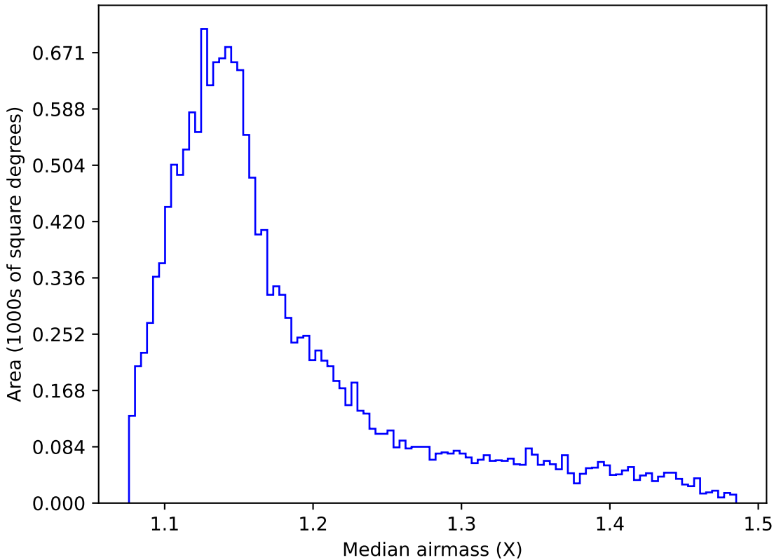
too_ignore_100_1v3.4_10yrs WFD g band: Median airmass
