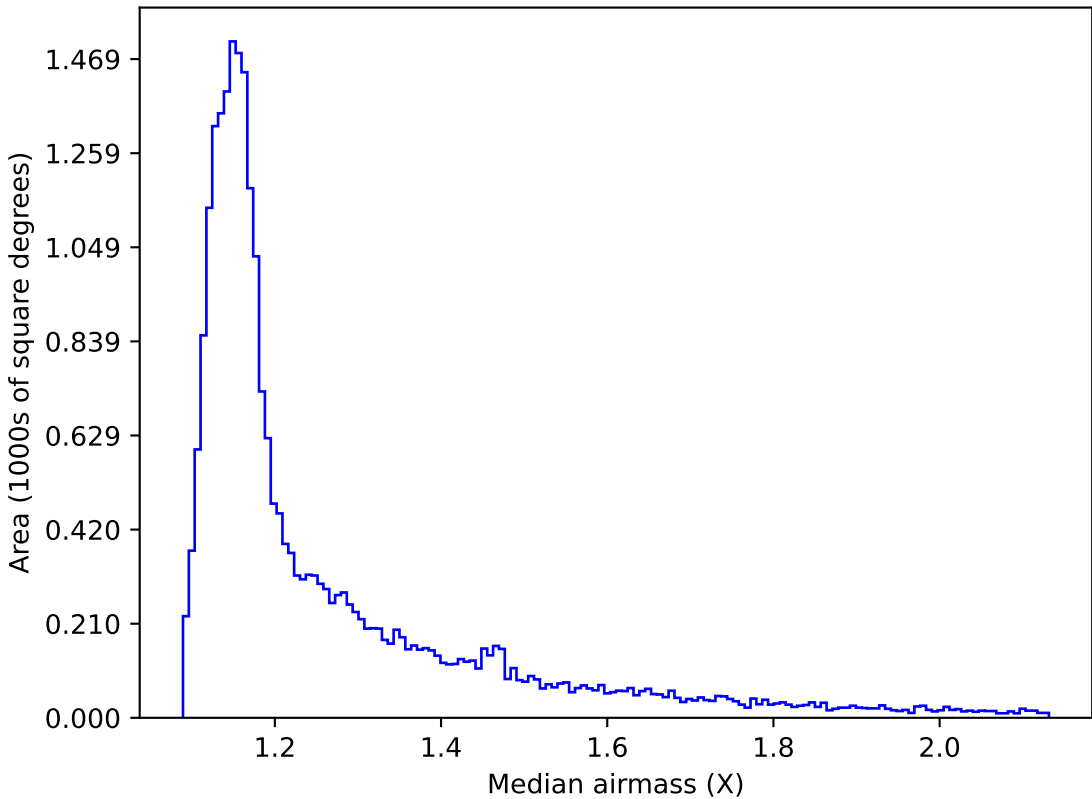
too_ignore_100_1v3.4_10yrs All sky z band: Median airmass
