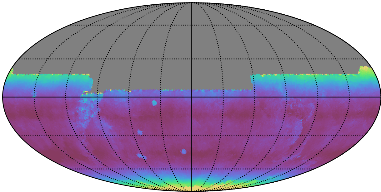
too_ignore_100_1v3.4_10yrs All sky y band: Median airmass
