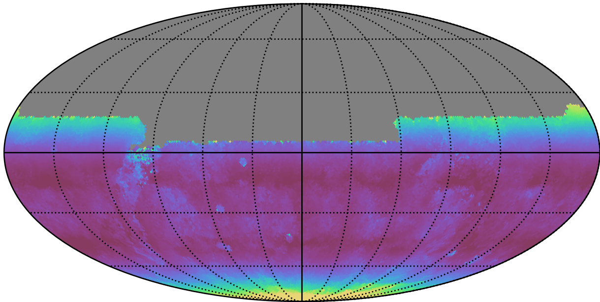
too_ignore_100_1v3.4_10yrs All sky u band: Median airmass
