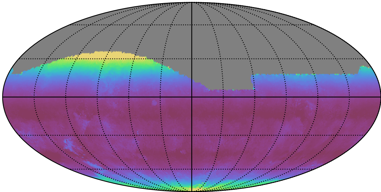
too_ignore_100_1v3.4_10yrs All sky g band: Median airmass
