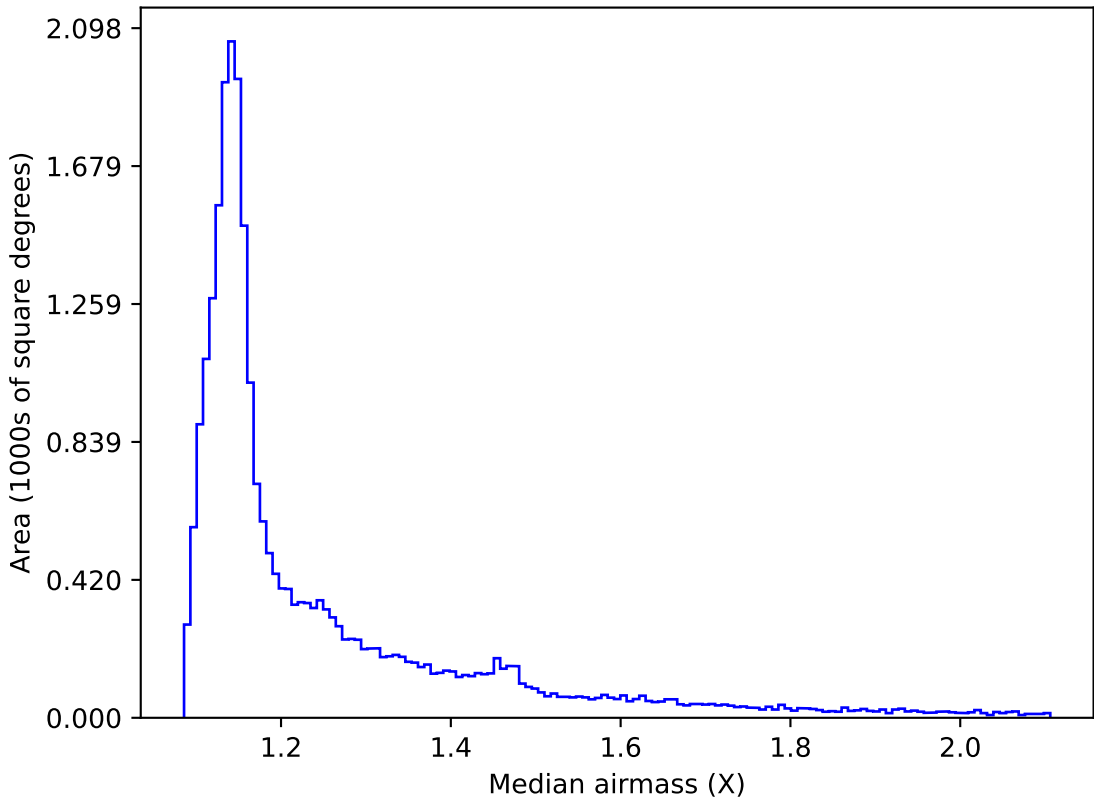
too_ignore_100_1v3.4_10yrs All sky all bands: Median airmass
