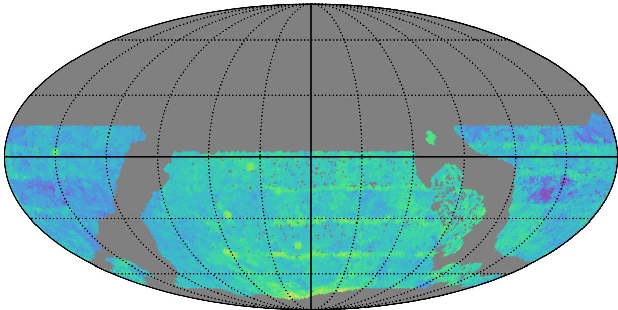
too_ignore_100_1v3.4_10yrs WFD z band: Median Season Length
