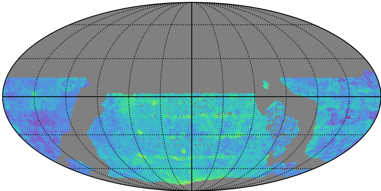
too_ignore_100_1v3.4_10yrs WFD y band: Median Season Length
