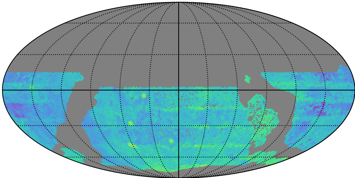
too_ignore_100_1v3.4_10yrs WFD r band: Median Season Length
