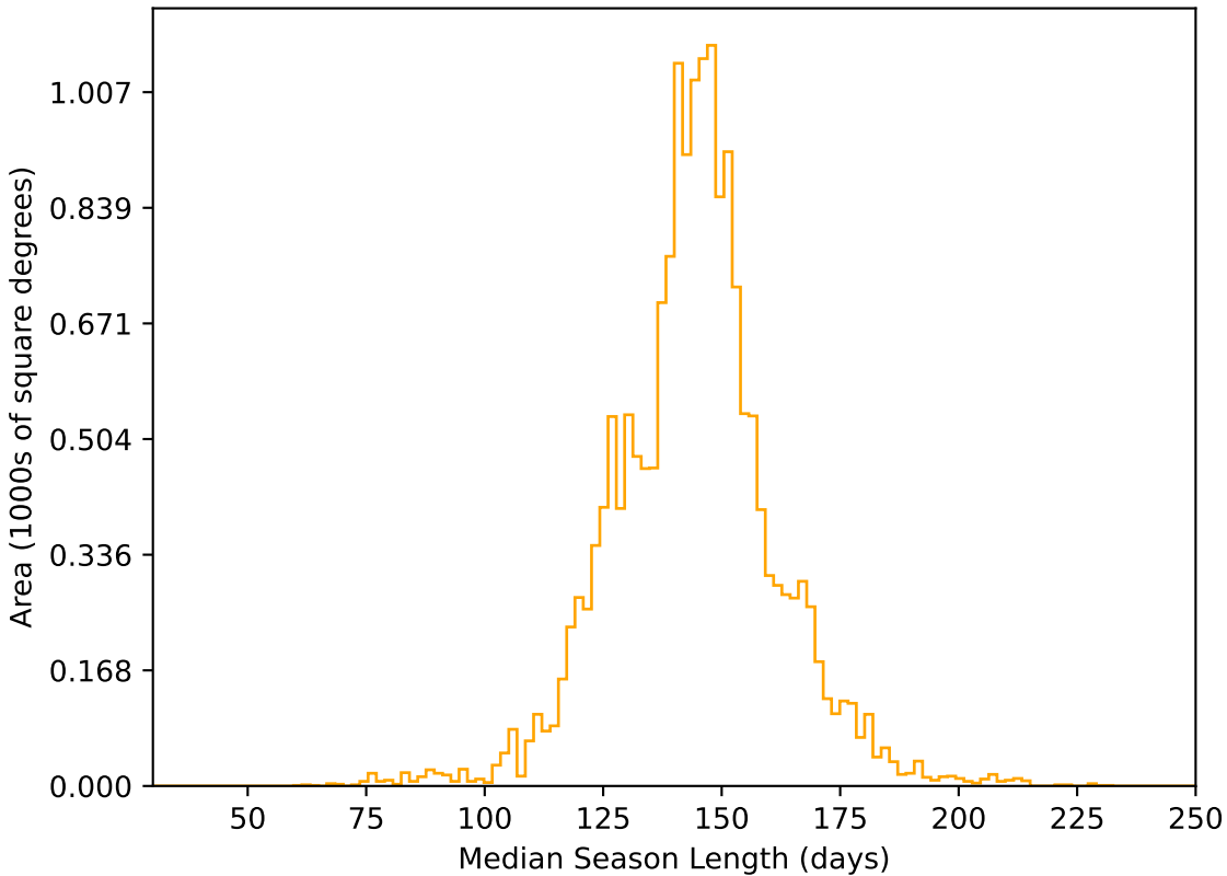
too_ignore_100_1v3.4_10yrs WFD r band: Median Season Length
