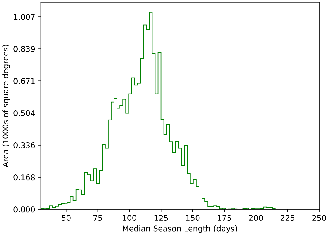
too_ignore_100_1v3.4_10yrs WFD g band: Median Season Length
