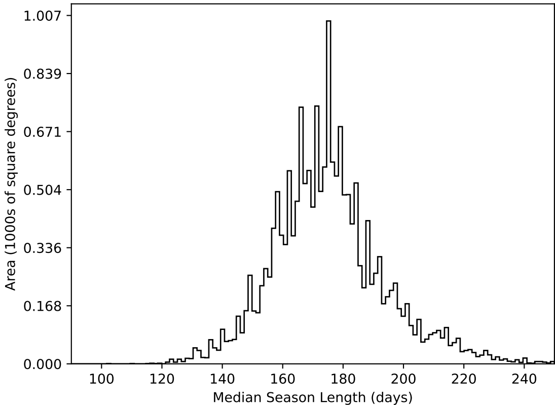
too_ignore_100_1v3.4_10yrs WFD all bands: Median Season Length
