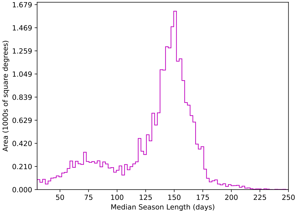
too_ignore_100_1v3.4_10yrs All sky z band: Median Season Length
