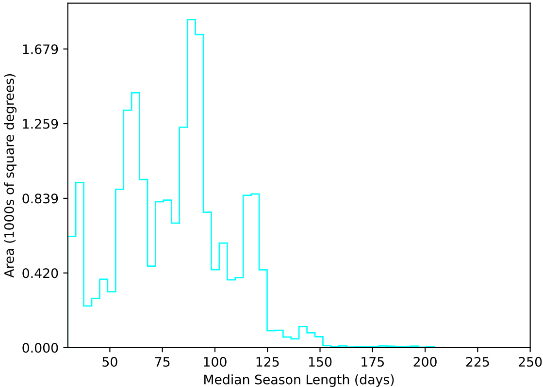
too_ignore_100_1v3.4_10yrs All sky u band: Median Season Length
