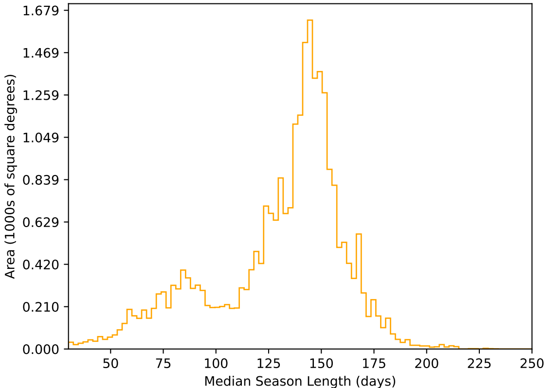
too_ignore_100_1v3.4_10yrs All sky r band: Median Season Length
