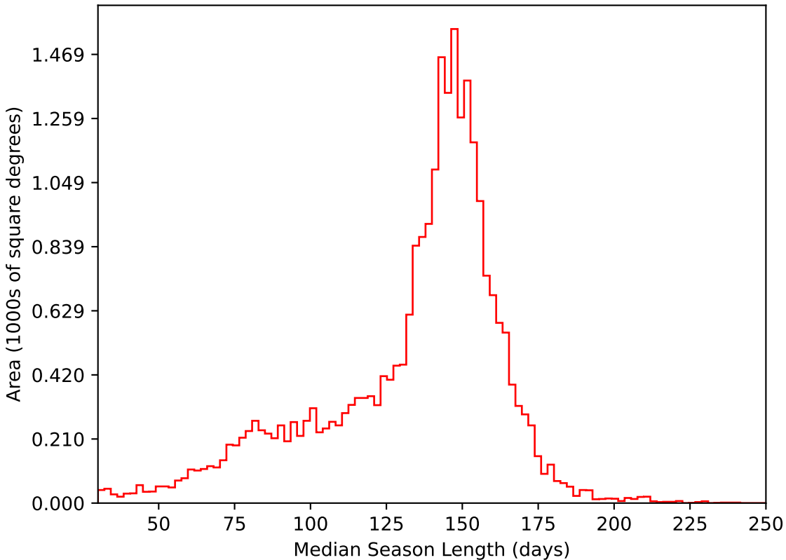
too_ignore_100_1v3.4_10yrs All sky i band: Median Season Length
