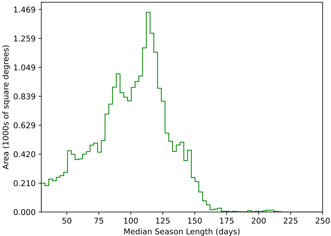
too_ignore_100_1v3.4_10yrs All sky g band: Median Season Length
