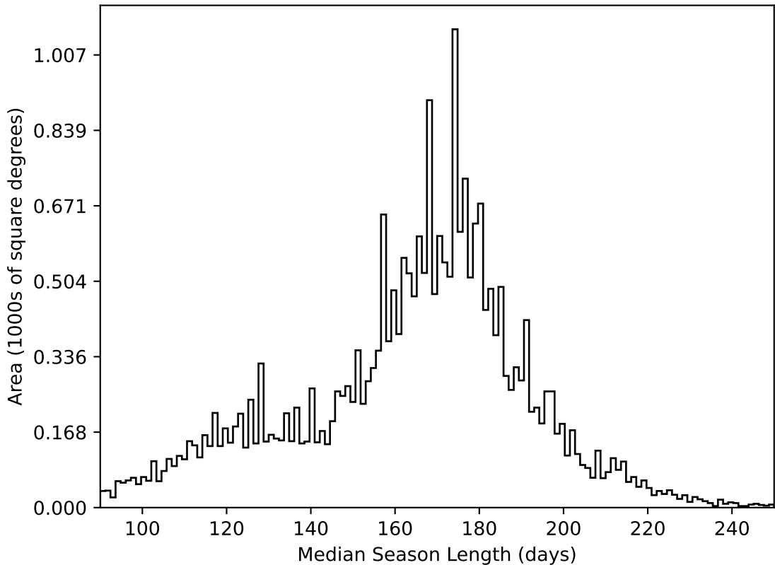
too_ignore_100_1v3.4_10yrs All sky all bands: Median Season Length
