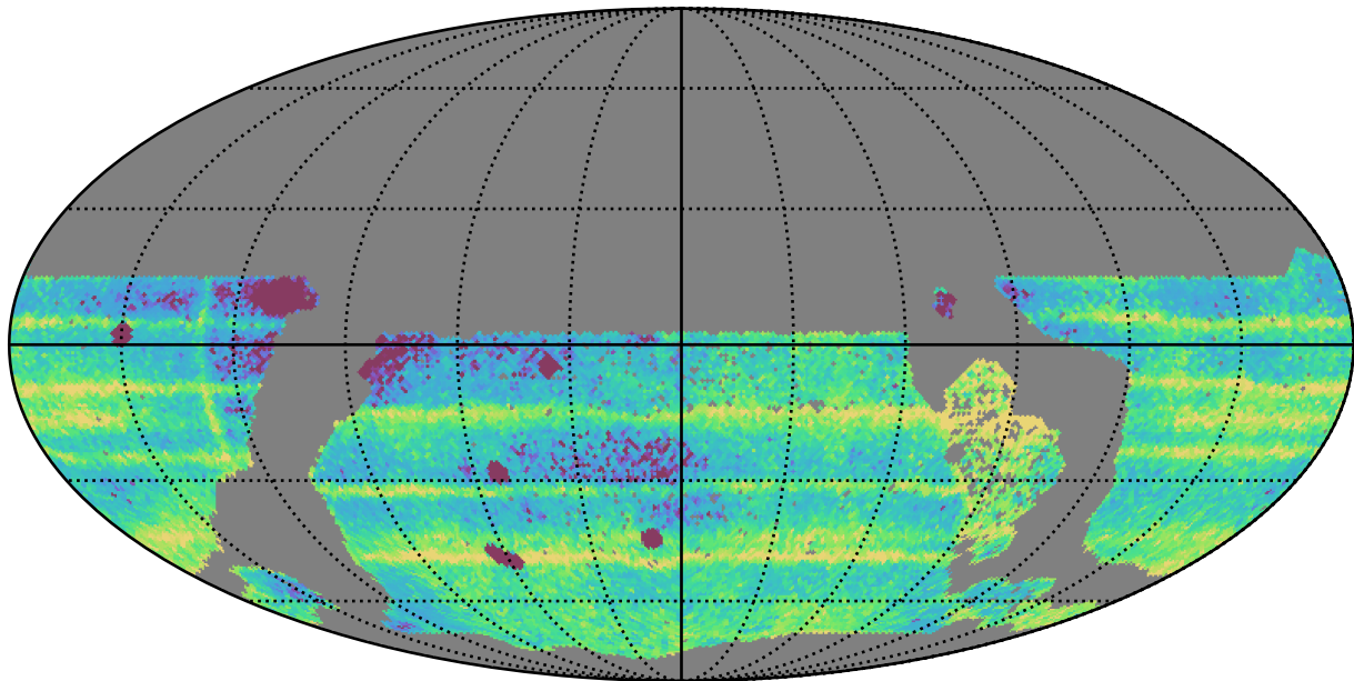
too_ignore_100_1v3.4_10yrs WFD: Median Intra-Night Gap
