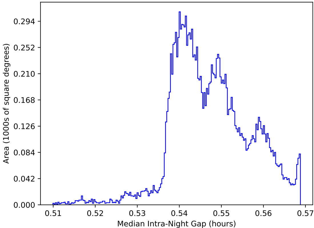
too_ignore_100_1v3.4_10yrs WFD: Median Intra-Night Gap
