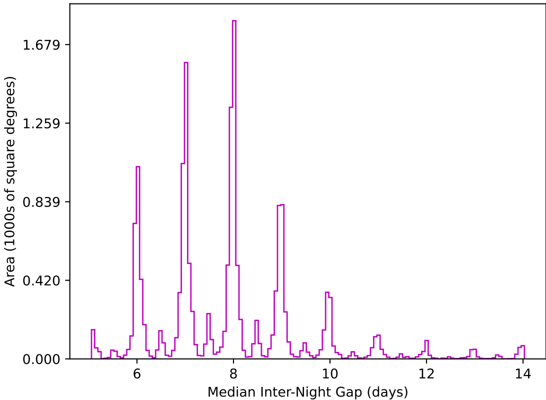
too_ignore_100_1v3.4_10yrs WFD z band: Median Inter-Night Gap
