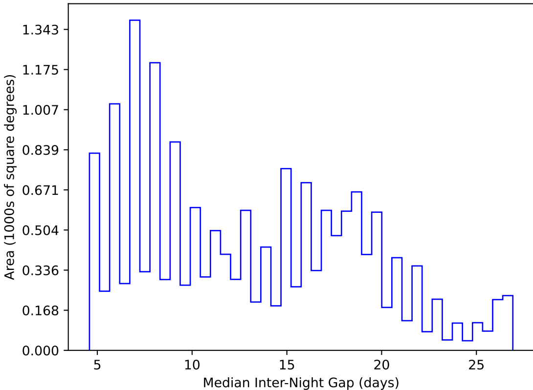
too_ignore_100_1v3.4_10yrs WFD y band: Median Inter-Night Gap
