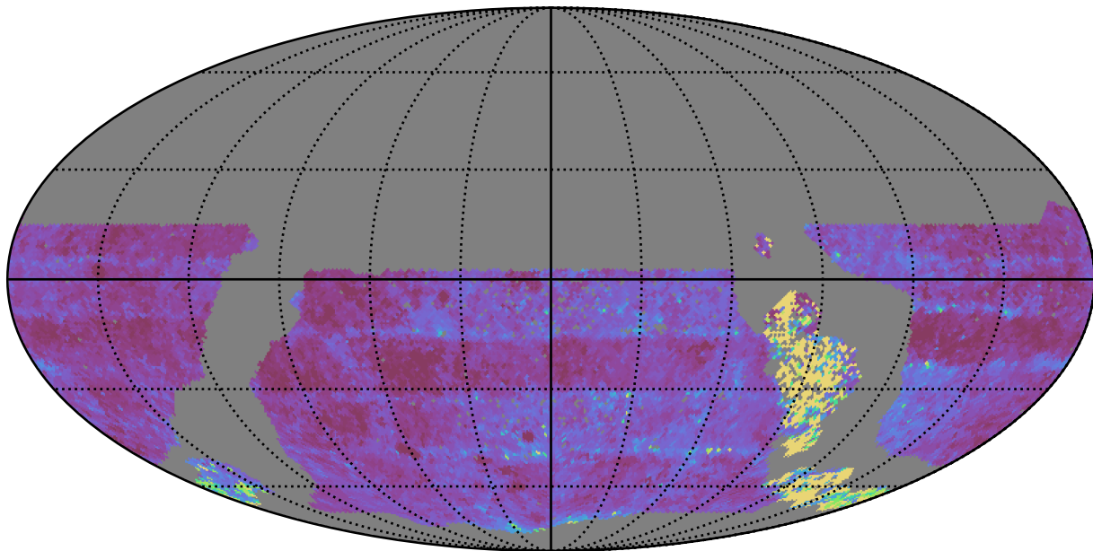
too_ignore_100_1v3.4_10yrs WFD u band: Median Inter-Night Gap
