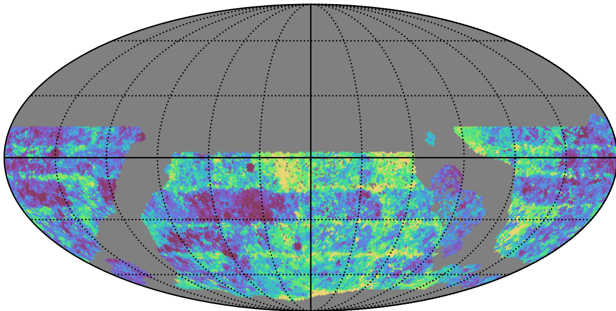
too_ignore_100_1v3.4_10yrs WFD g band: Median Inter-Night Gap
