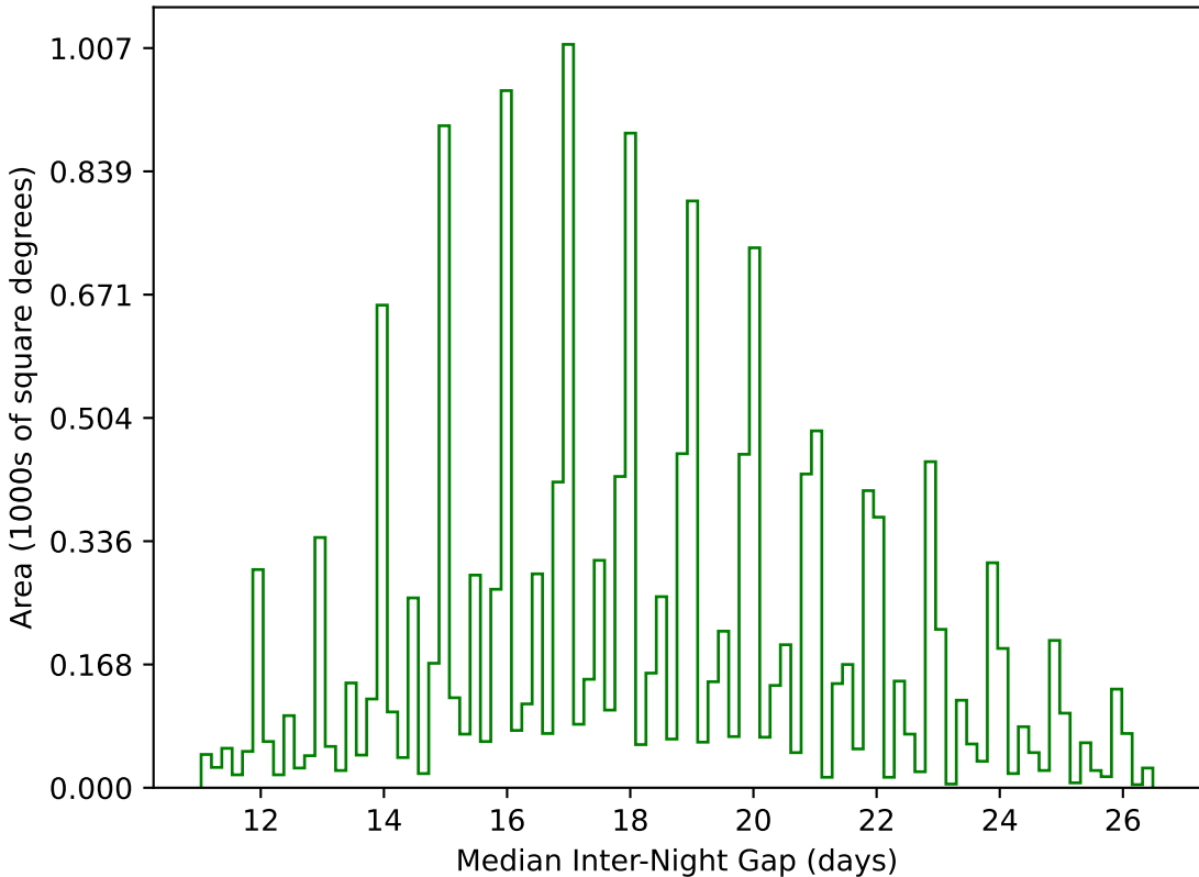
too_ignore_100_1v3.4_10yrs WFD g band: Median Inter-Night Gap
