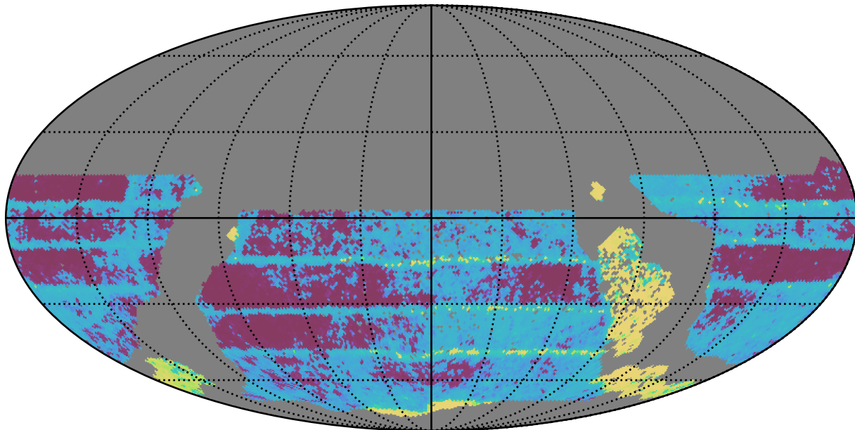
too_ignore_100_1v3.4_10yrs WFD all bands: Median Inter-Night Gap
