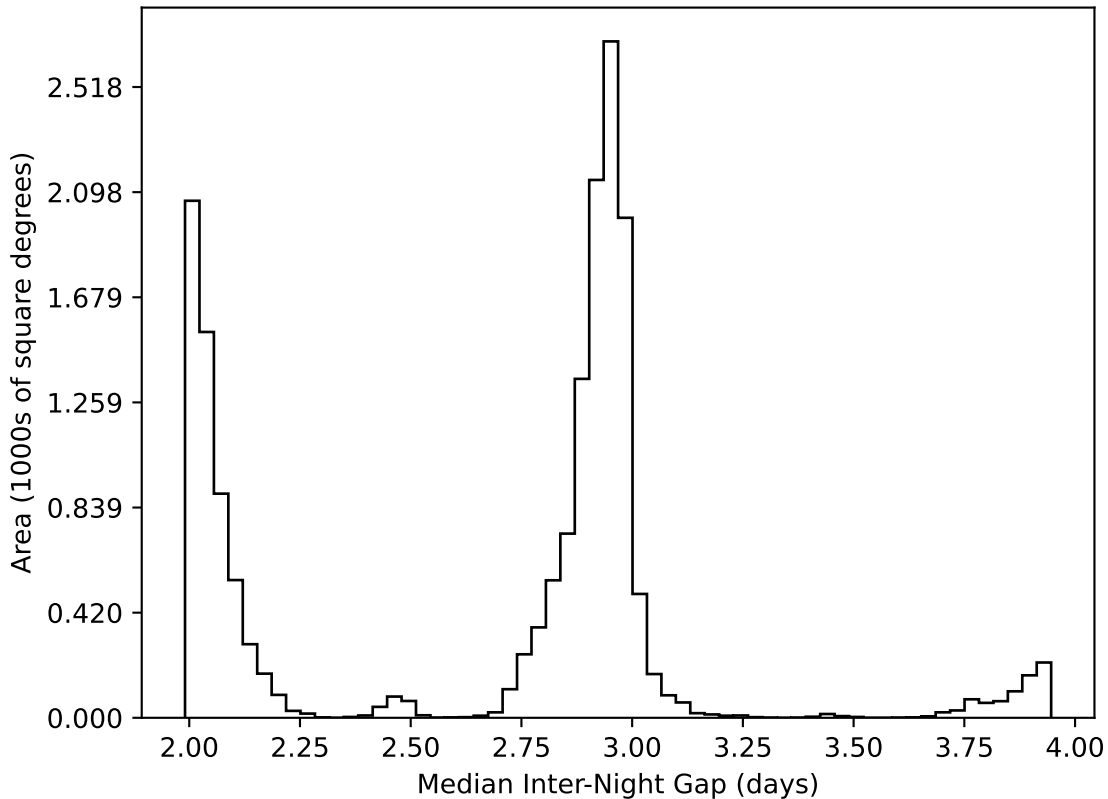
too_ignore_100_1v3.4_10yrs WFD all bands: Median Inter-Night Gap
