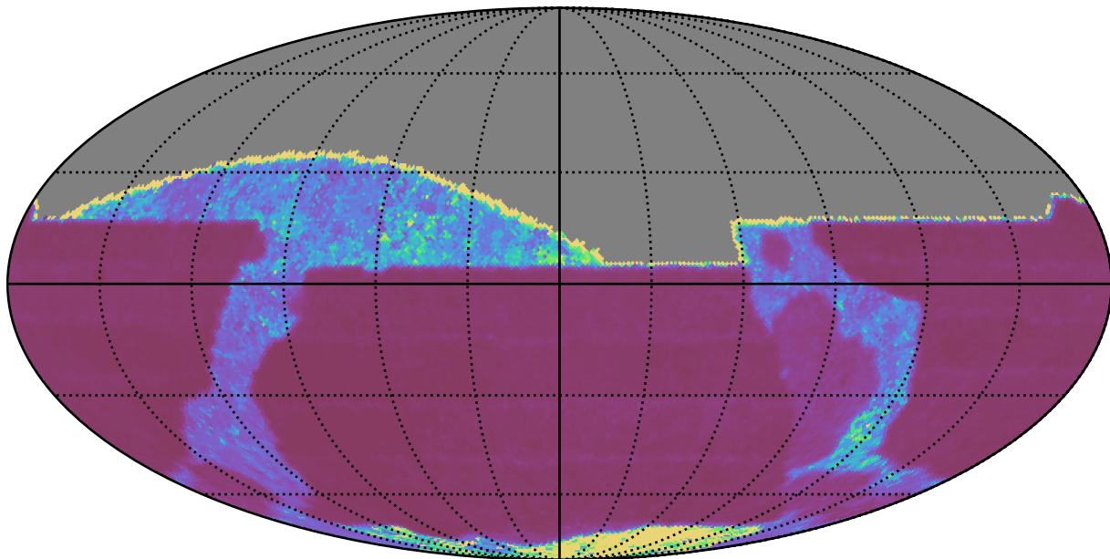
too_ignore_100_1v3.4_10yrs All sky z band: Median Inter-Night Gap
