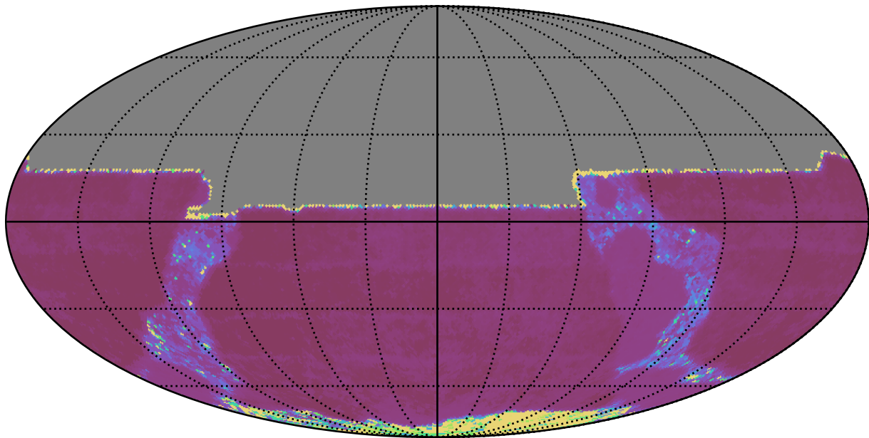
too_ignore_100_1v3.4_10yrs All sky y band: Median Inter-Night Gap
