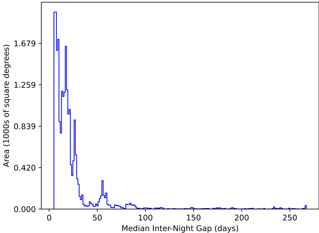
too_ignore_100_1v3.4_10yrs All sky y band: Median Inter-Night Gap
