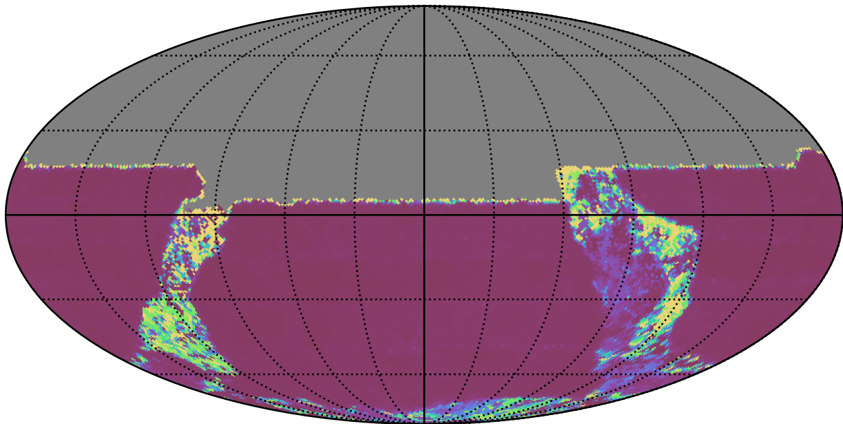
too_ignore_100_1v3.4_10yrs All sky u band: Median Inter-Night Gap
