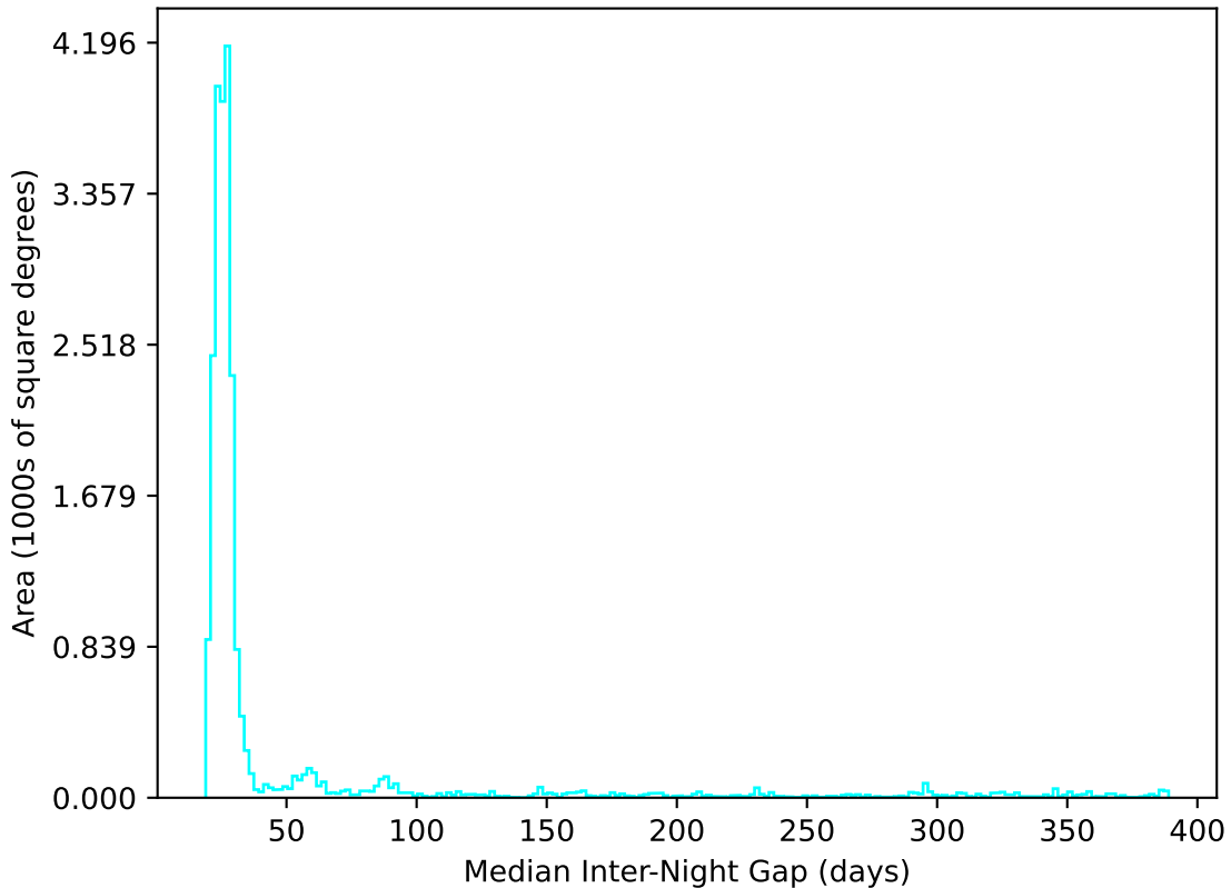
too_ignore_100_1v3.4_10yrs All sky u band: Median Inter-Night Gap
