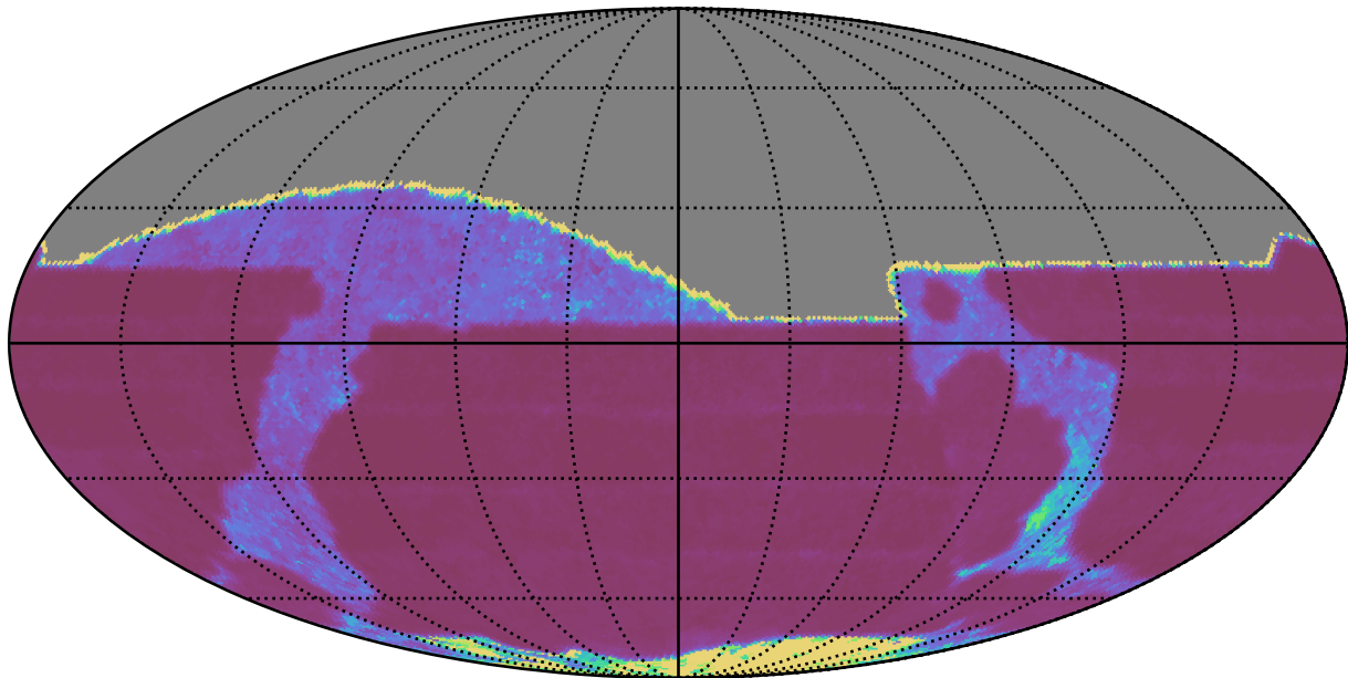
too_ignore_100_1v3.4_10yrs All sky r band: Median Inter-Night Gap
