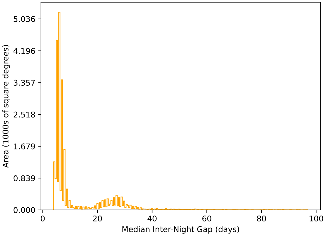
too_ignore_100_1v3.4_10yrs All sky r band: Median Inter-Night Gap
