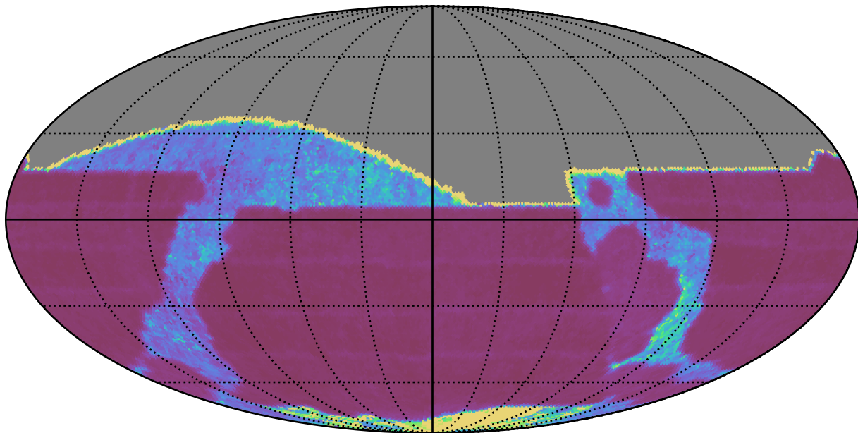
too_ignore_100_1v3.4_10yrs All sky i band: Median Inter-Night Gap
