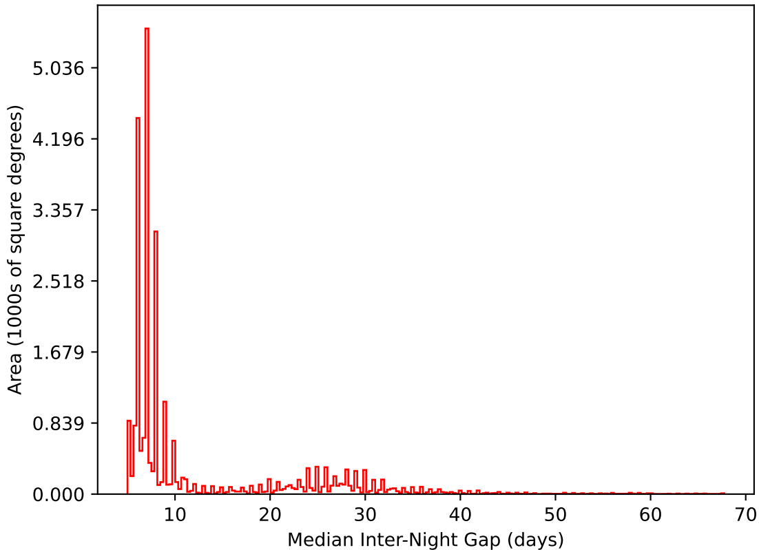
too_ignore_100_1v3.4_10yrs All sky i band: Median Inter-Night Gap
