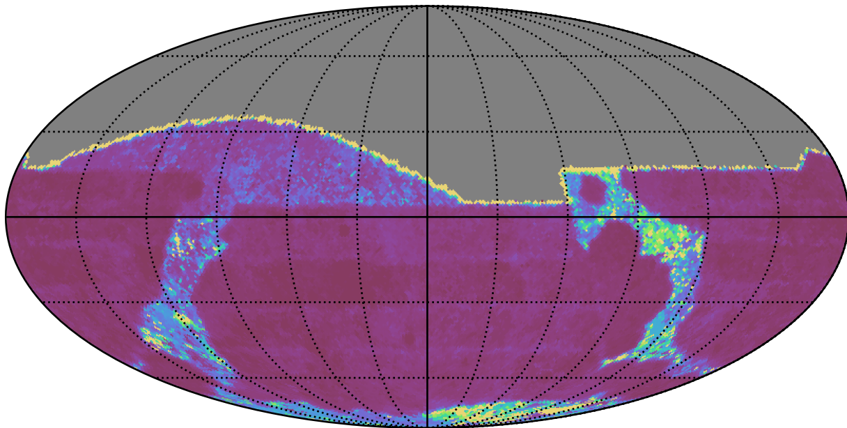
too_ignore_100_1v3.4_10yrs All sky g band: Median Inter-Night Gap
