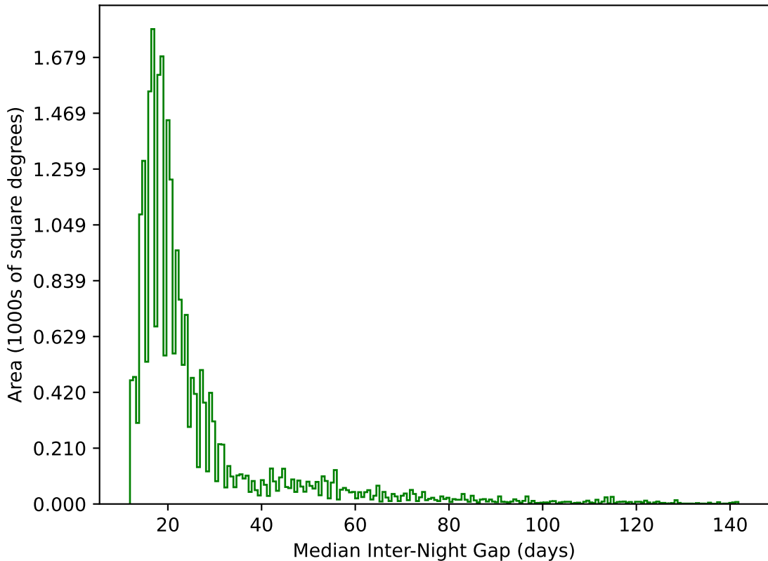
too_ignore_100_1v3.4_10yrs All sky g band: Median Inter-Night Gap
